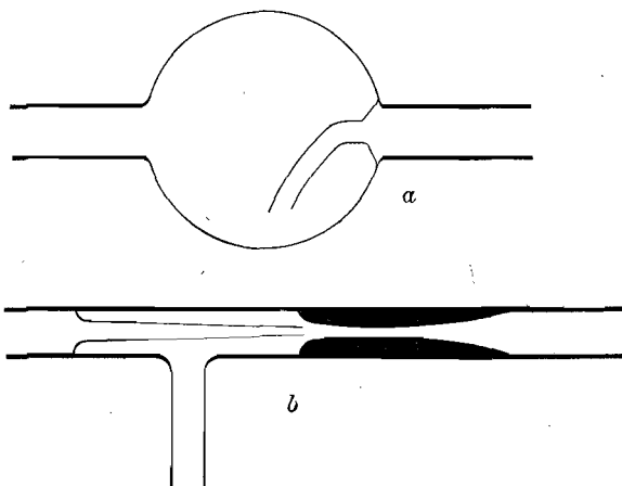
FIG. 13.— a , Kjeldahl trap; b , suction pump on smaller tubing.
