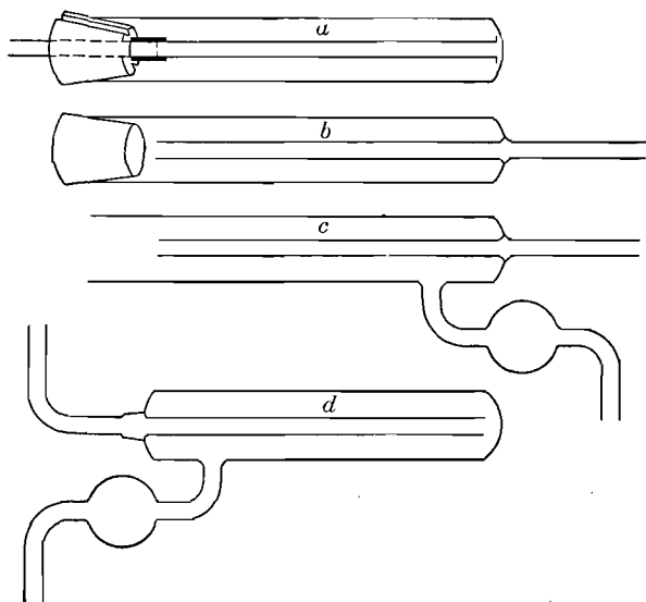
FIG. 11.—Gas-washing tube.
