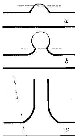
FIG. 7.—The "tee" tube.
