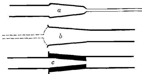
FIG. 17.—Ground joint.
