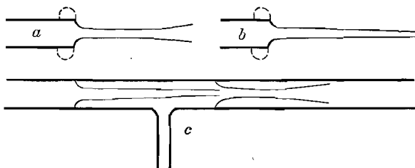
FIG. 12.—Suction pump.
